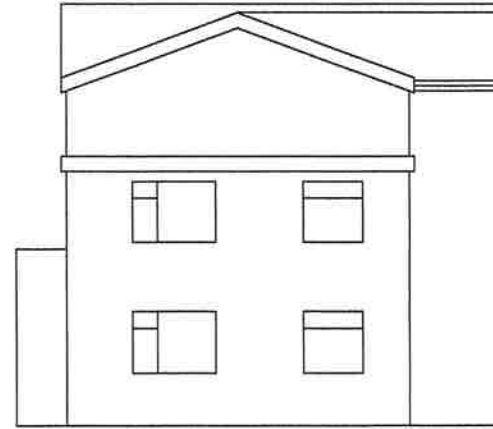
REAR ELEVATION EXISTING & PROPOSED (NO CHANGES)
