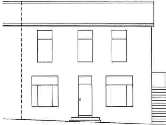
FRONT ELEVATION EXISTING & PROPOSED (NO CHANGES)
