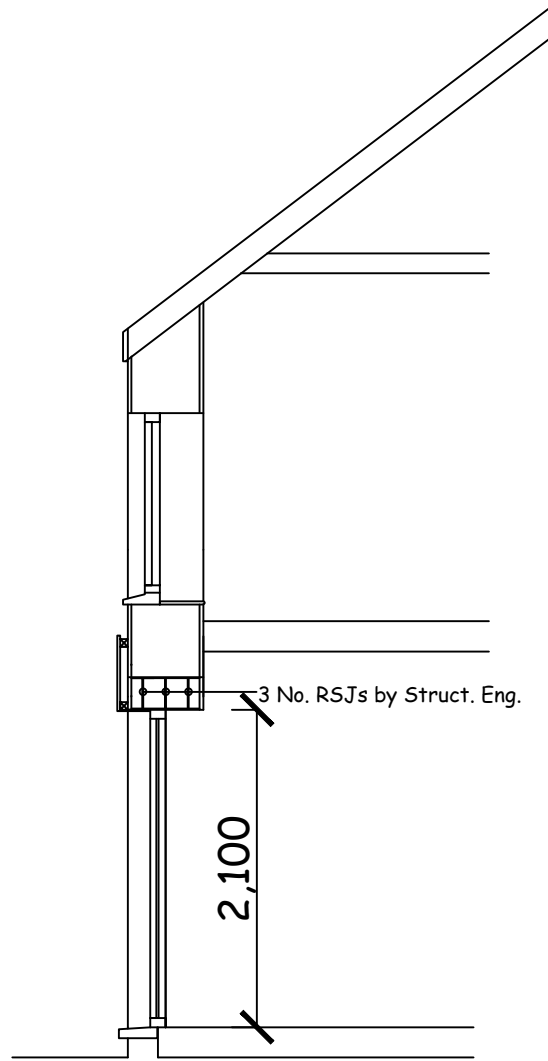
PROPOSED SECTION 1:50
