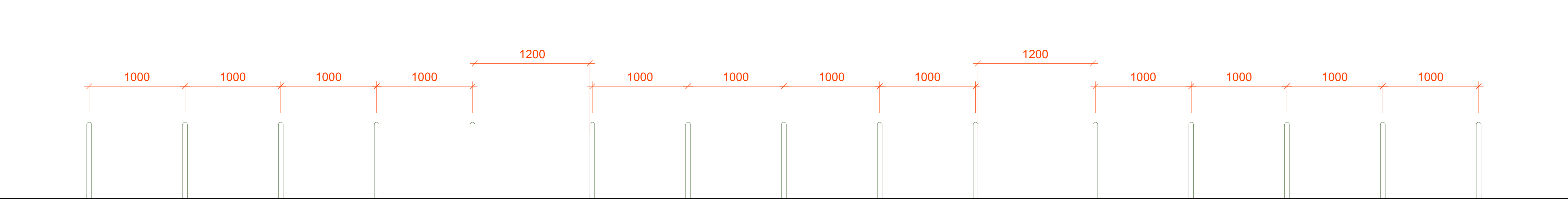
00211.1 - MAIN CARPARK - CYCLE STAND ELEVATION SCALE 1:25 @ A1, 1:50 @A3
