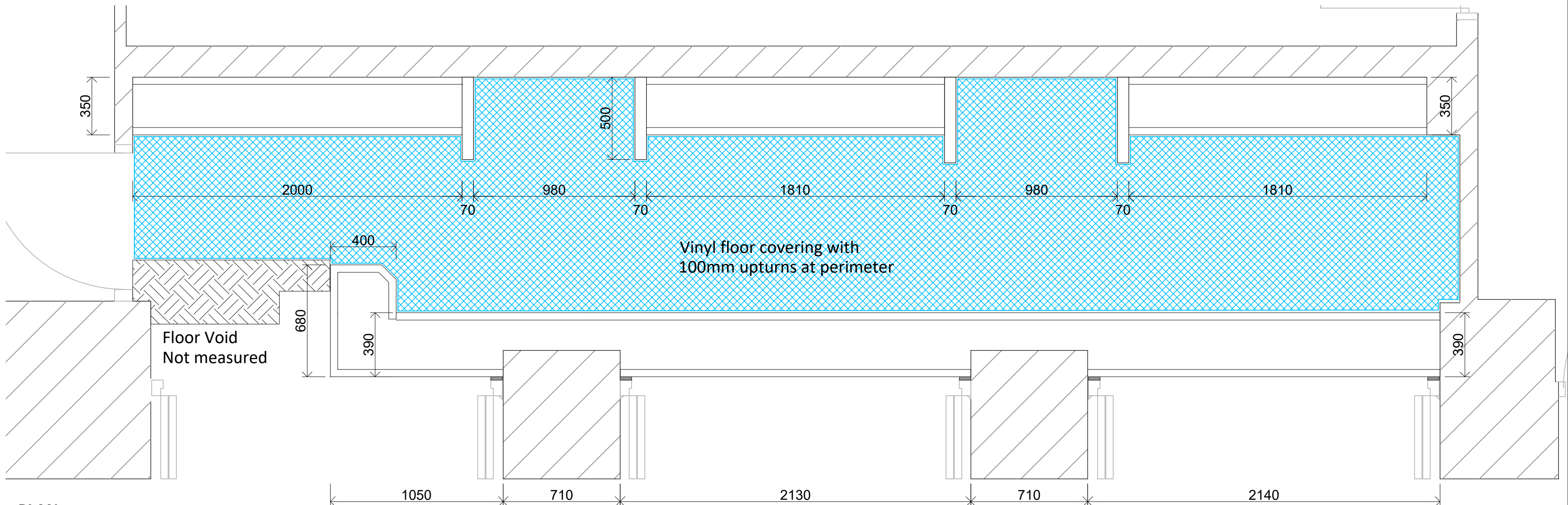
PLAN Proposed Primary Fixings
