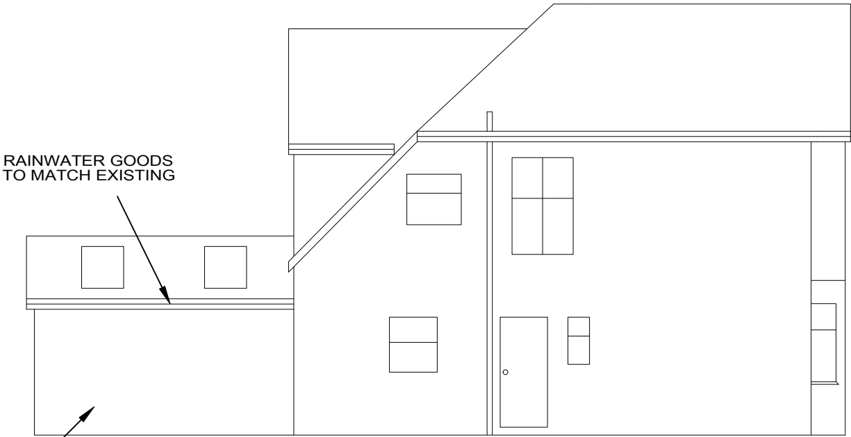
RIGHT SIDE ELEVATION PROPOSED
