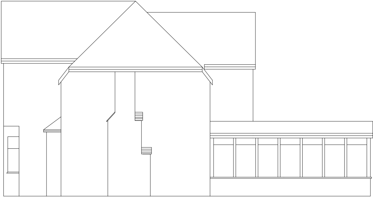
LEFT SIDE ELEVATION EXISTING
