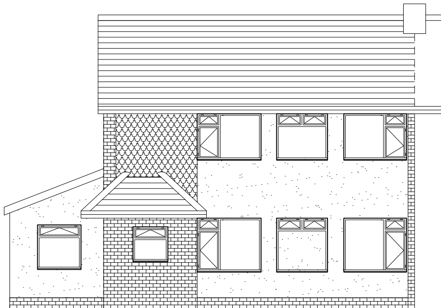
FRONT ELEVATION EXISTING
