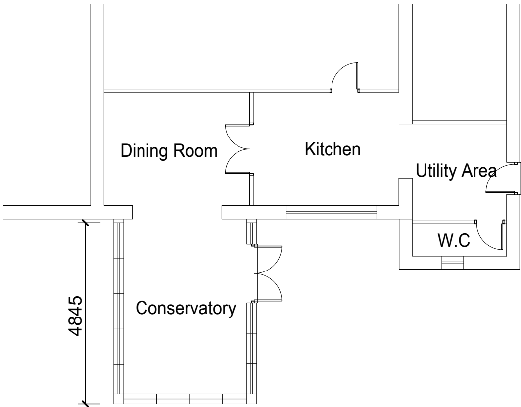
Partial Ground Floor Plan Existing
