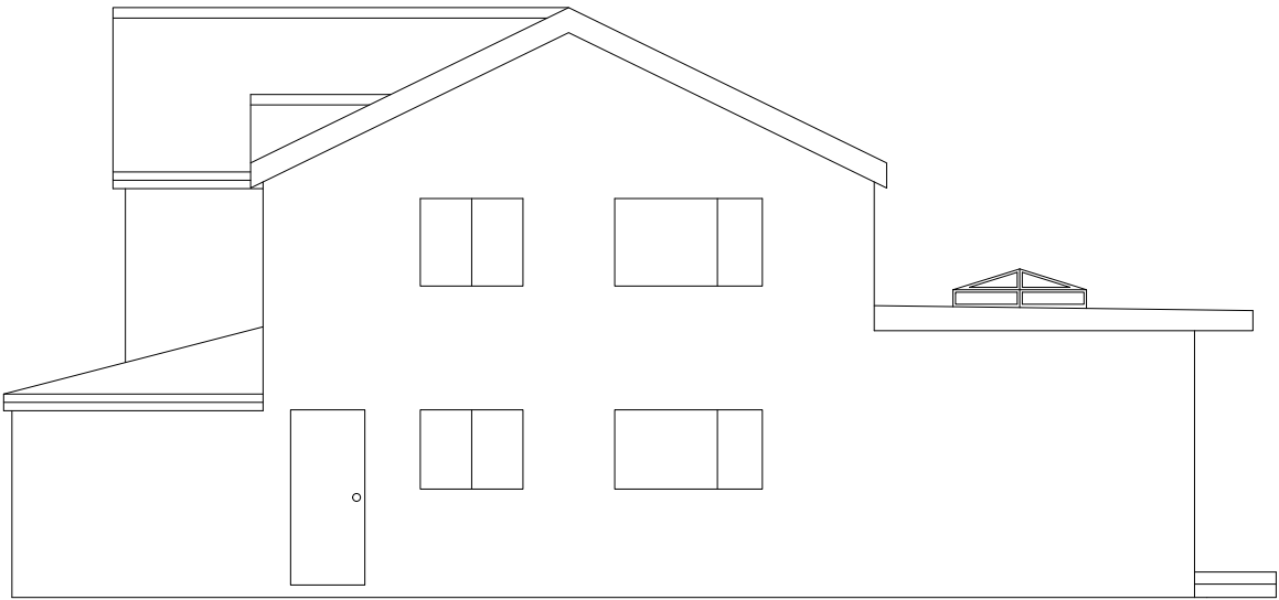
LEFT SIDE ELEVATION PROPOSED
