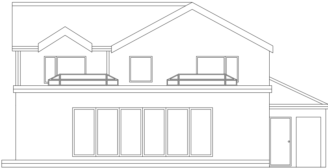
REAR ELEVATION PROPOSED
