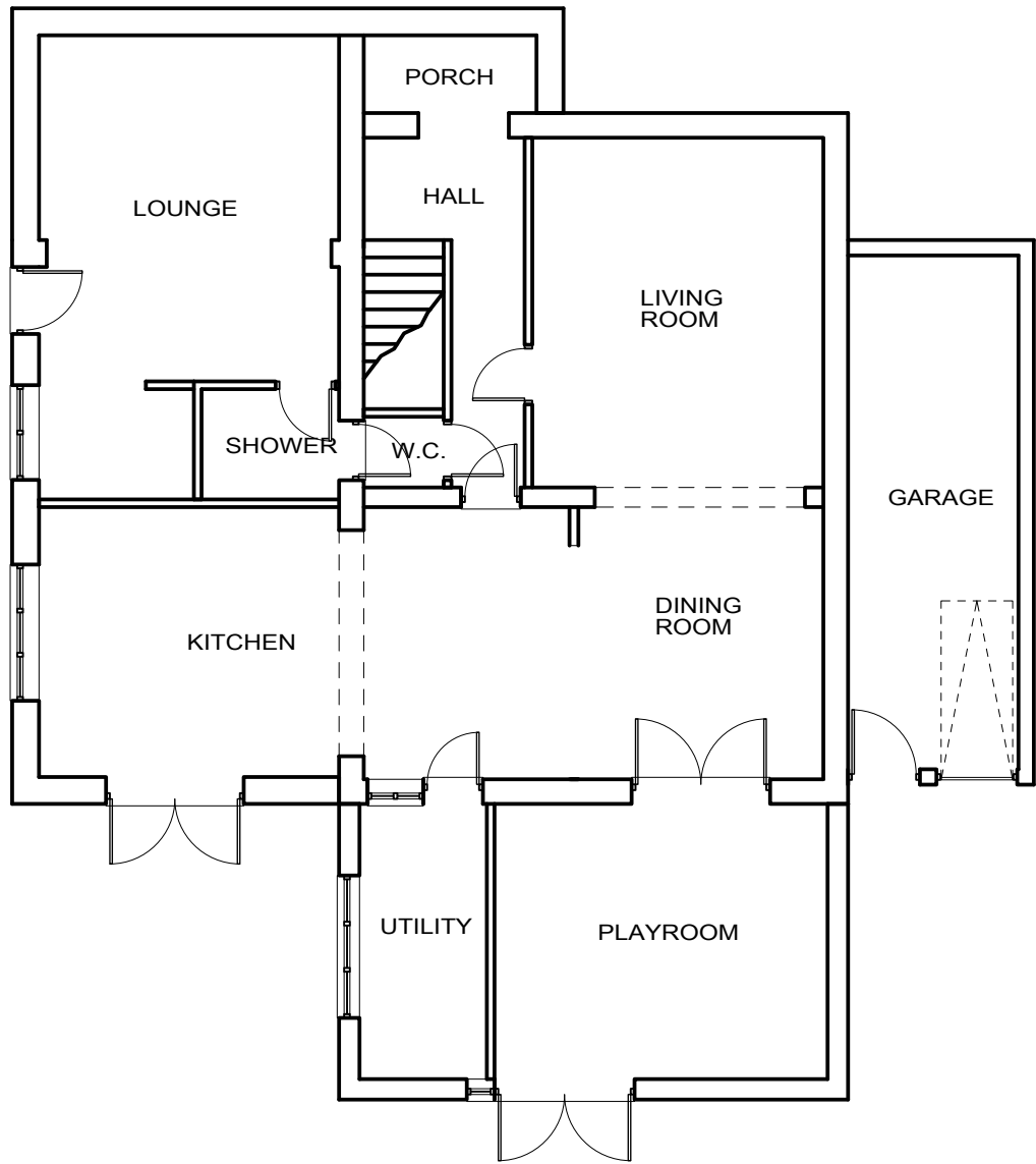
GROUND FLOOR PLANS EXISTING
