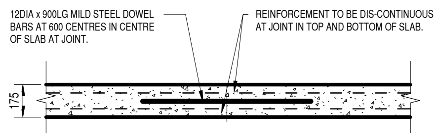
SLAB CONSTRUCTION JOINT (CJ)
