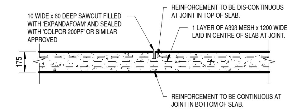
SLAB TRANSVERSE JOINT (TJ)
