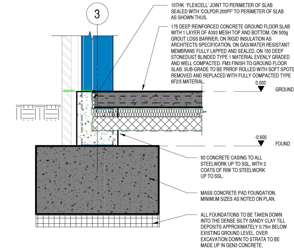
TYPICAL EDGE DETAIL
