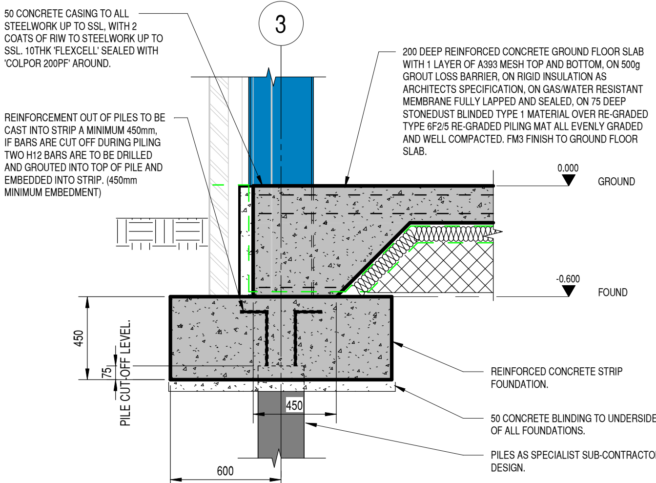
TYPICAL EDGE DETAIL (1 : 20)
