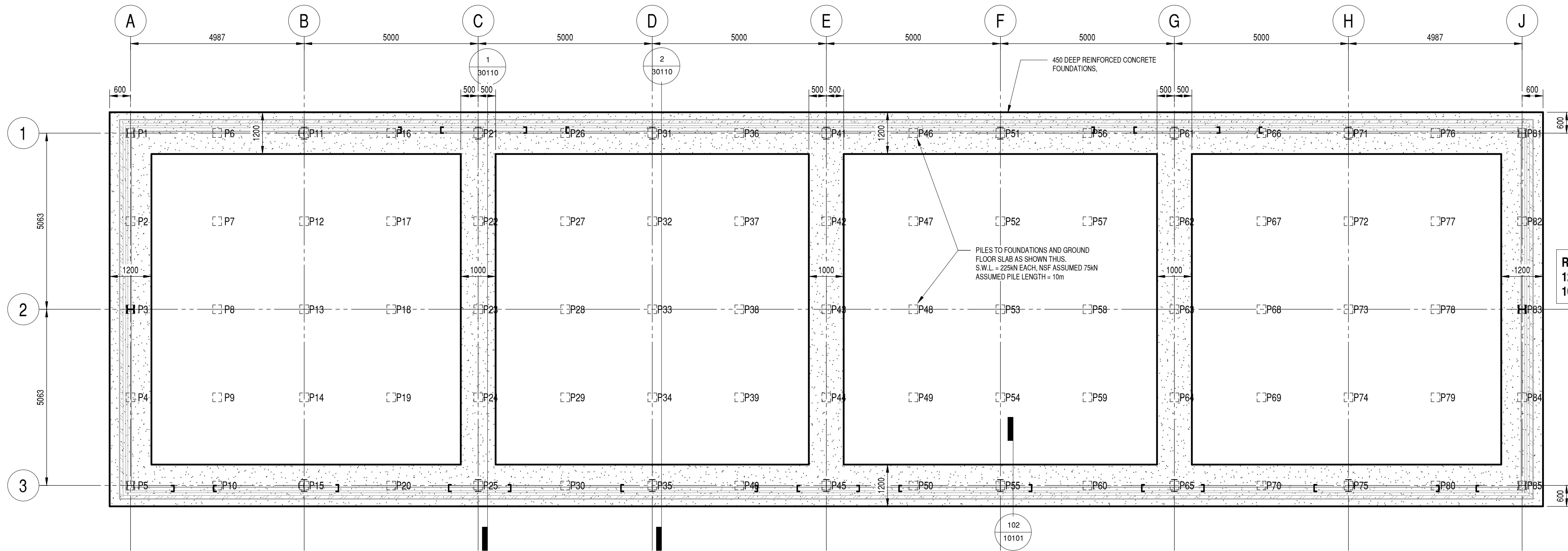
PLAN ON FOUNDATIONS (1 : 75)
