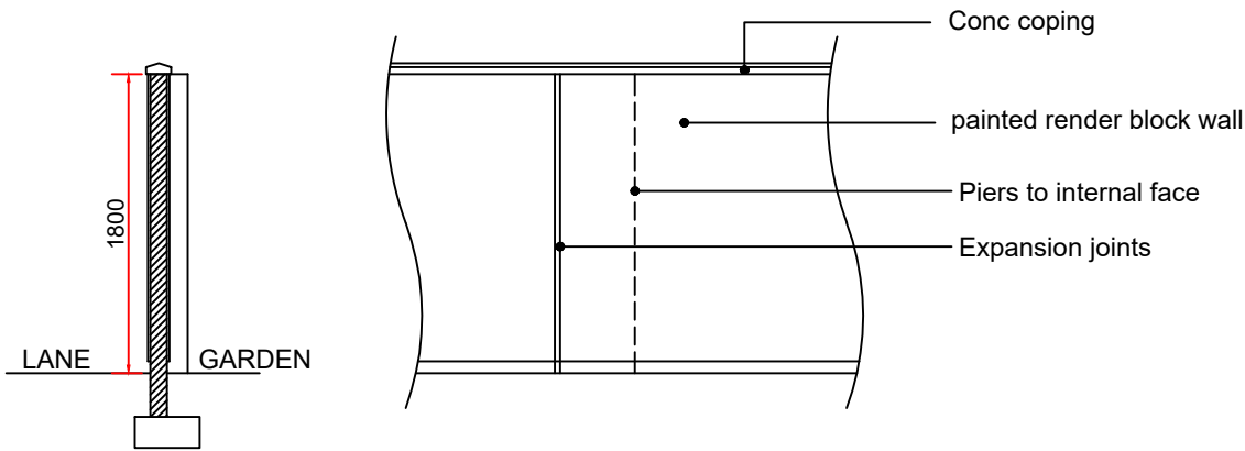
REAR WALL DETAIL
