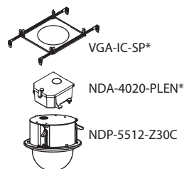
In-ceiling mount
