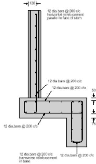
Reinforcement details
