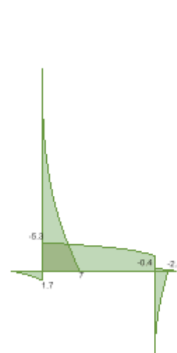
Bending moment - Combination No.1 - kNm/m
