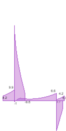
Shear force - Combination No.1 - kN/m
