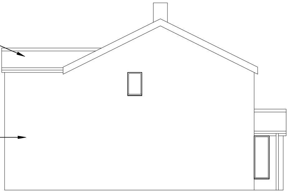
LEFT SIDE ELEVATION PROPOSED
