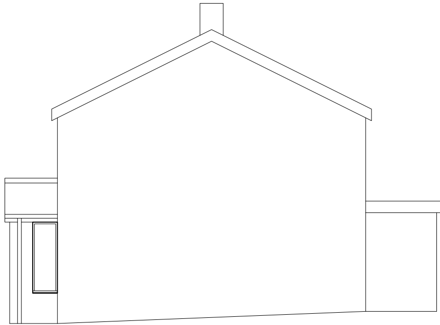
RIGHT SIDE ELEVATION EXISTING
