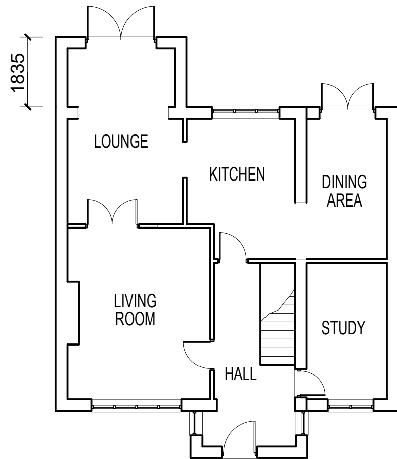
GROUND FLOOR PLAN EXISTING
