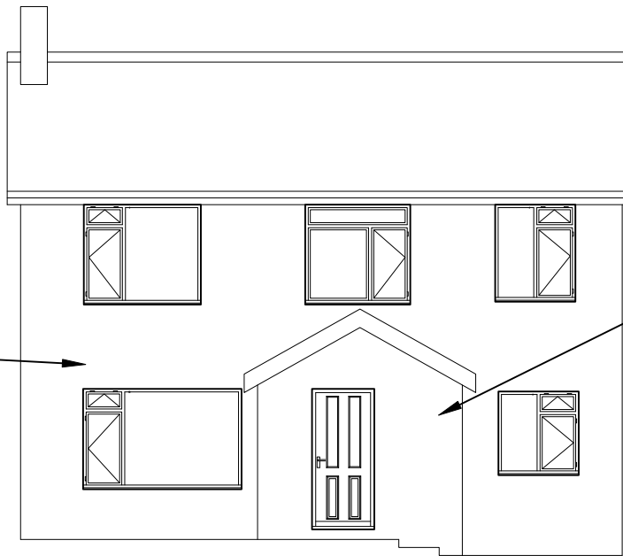
FRONT ELEVATION PROPOSED
