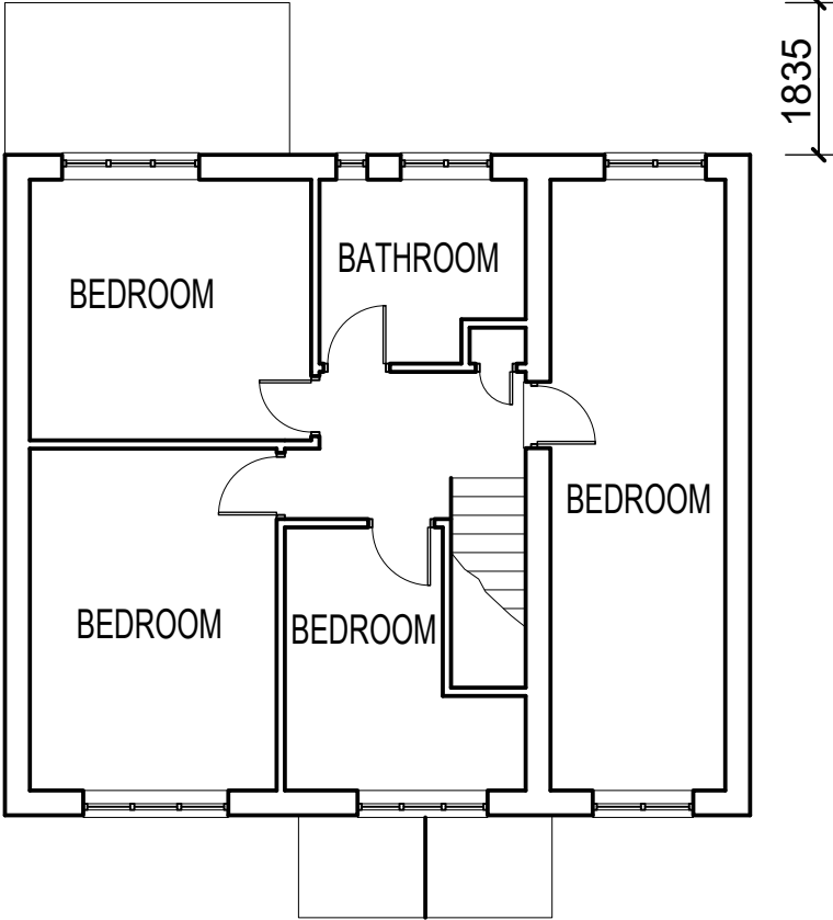
FIRST FLOOR PLAN EXISTING
