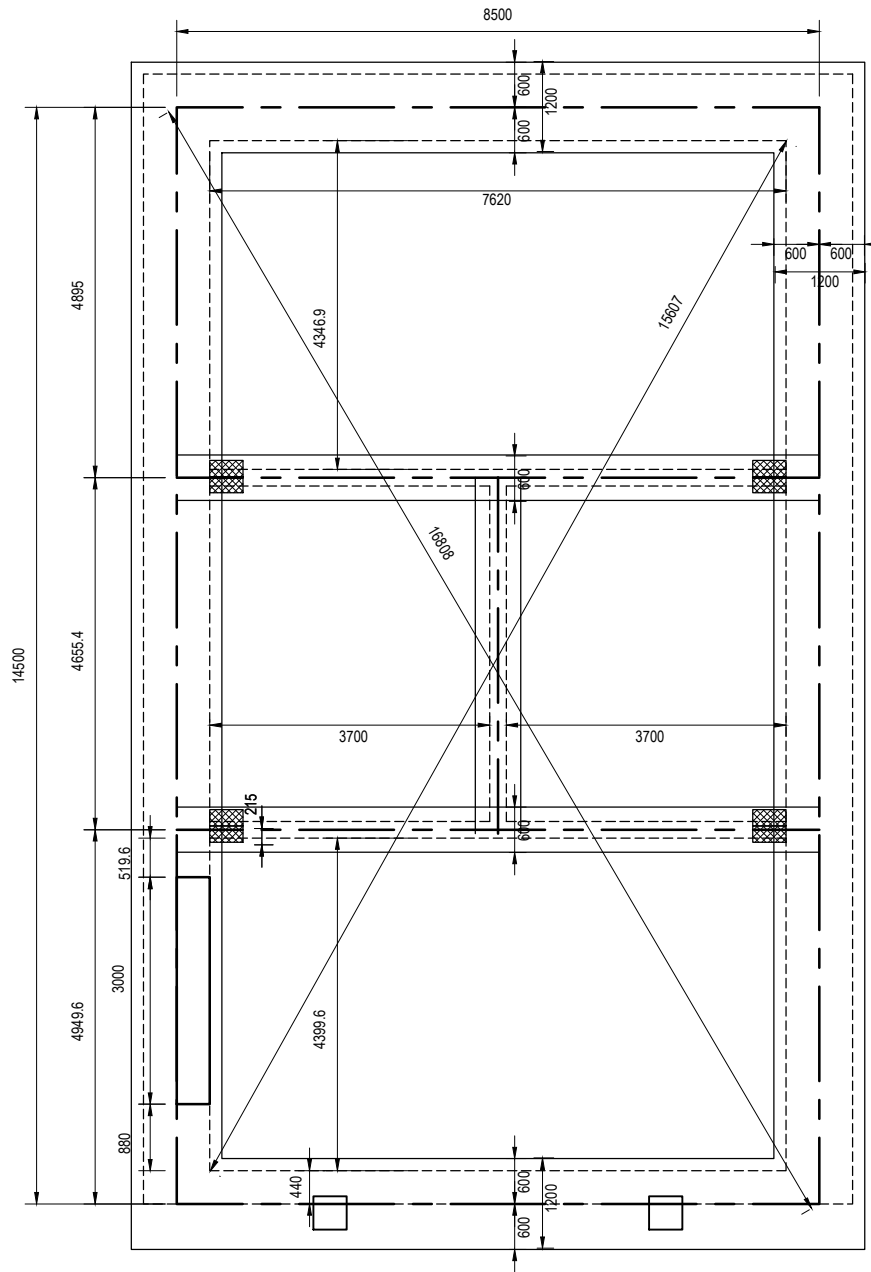
Foundation Plan Scale 1-100
