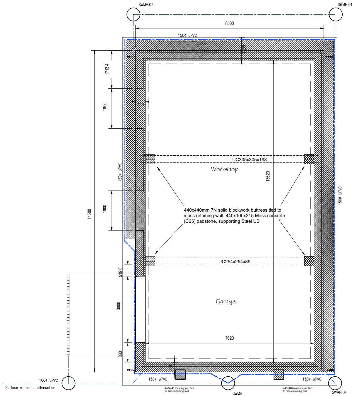
Basement Floor Plan Scale 1-100
