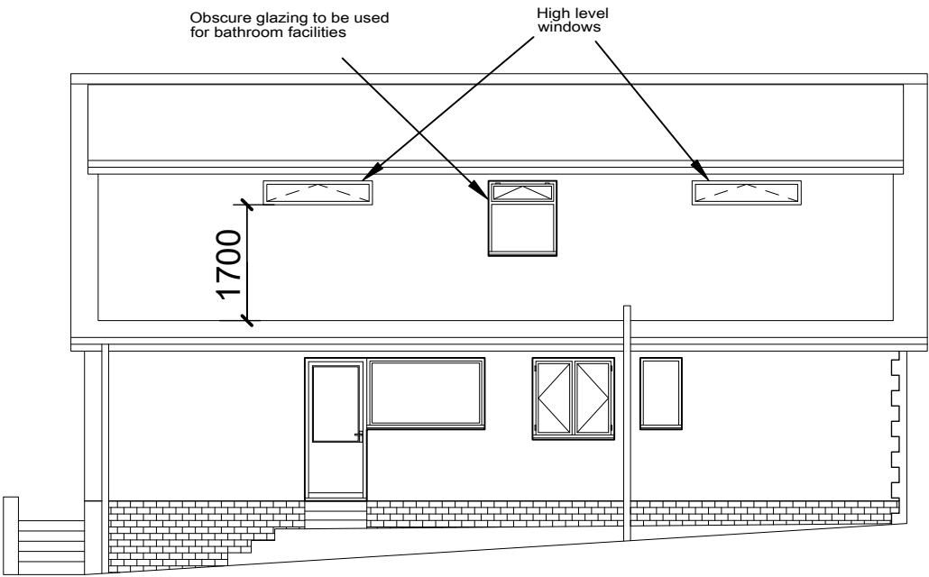
LEFT SIDE ELEVATION PROPOSED
