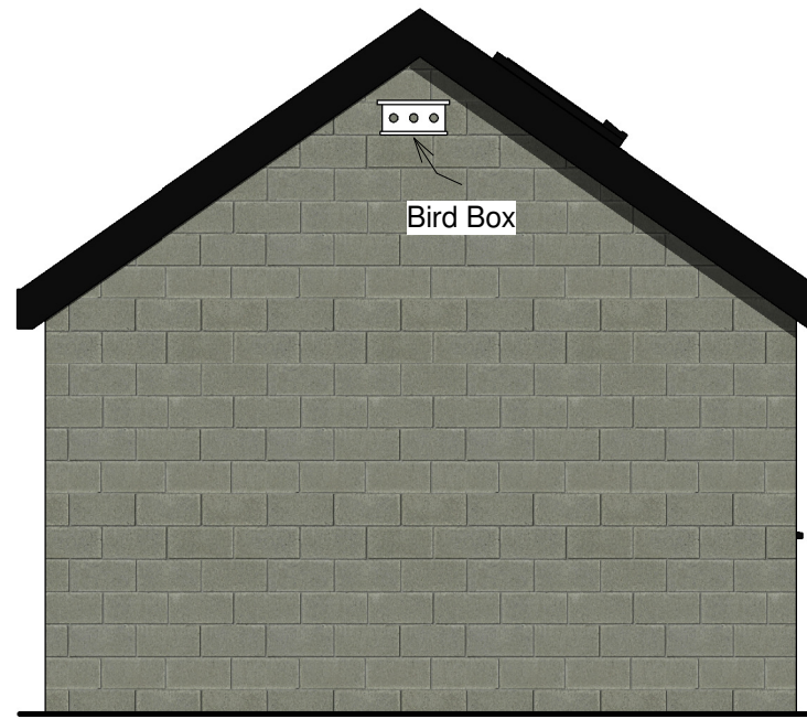
3 Left Elevation 1 : 50
