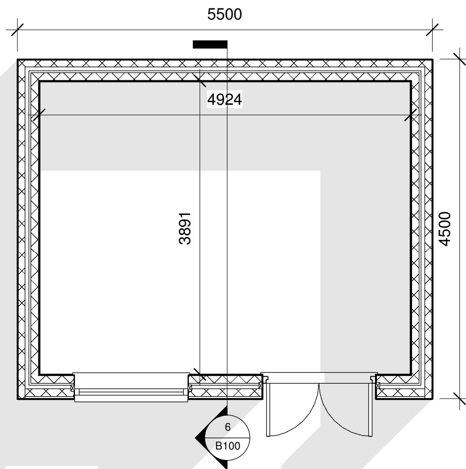
1 Proposed Floor Plan 1 : 50
