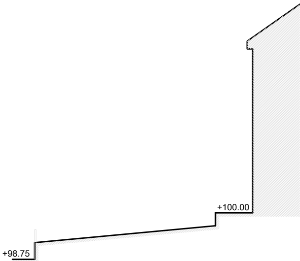
Existing Side Section / Elevation
