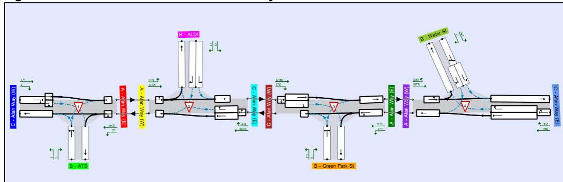
Figure 7.17 – Junctions 10 Linked Model Layout
