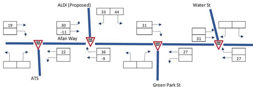
Figure 7.8 – Total ALDI Development Trip Assignment
