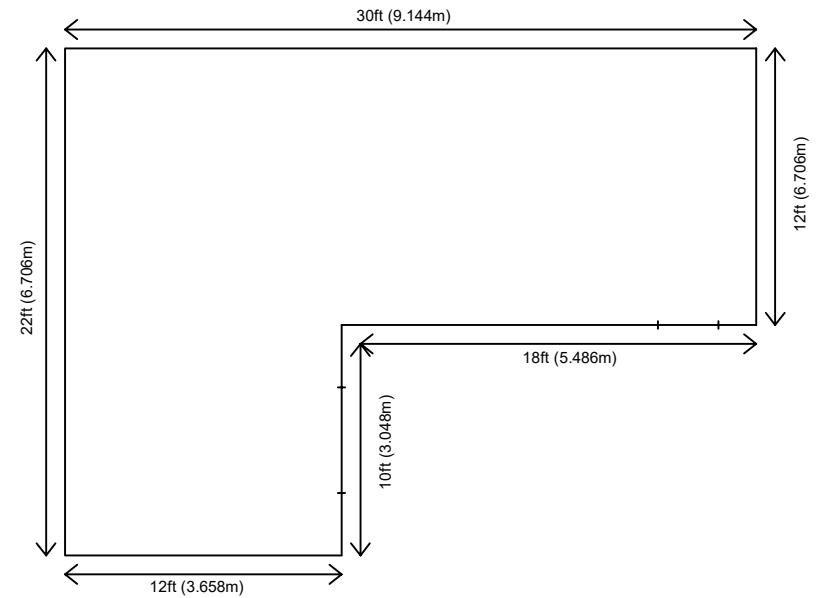
Floor plan after
