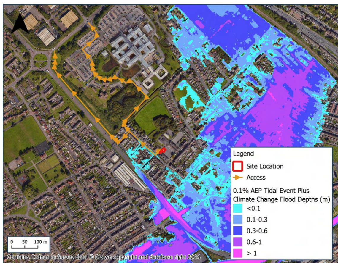
Figure 5-5 Access and Egress within the 0.1% AEP plus climate change tidal event
