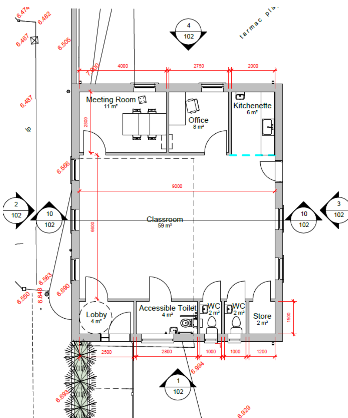
Figure 2-4: Extract of development proposals (Neath Port Talbot Borough Council)
