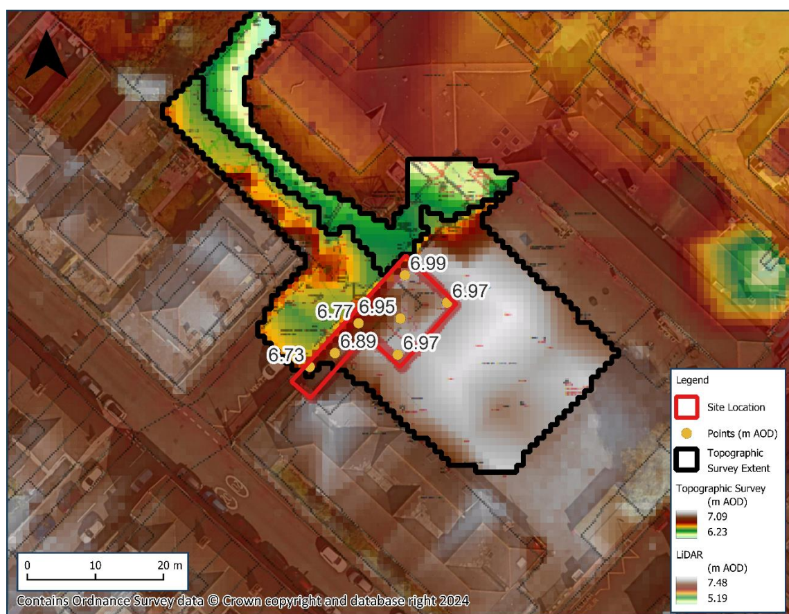
Figure 2-2: Site Specific Topographic Data from NPTCBC with sample points
