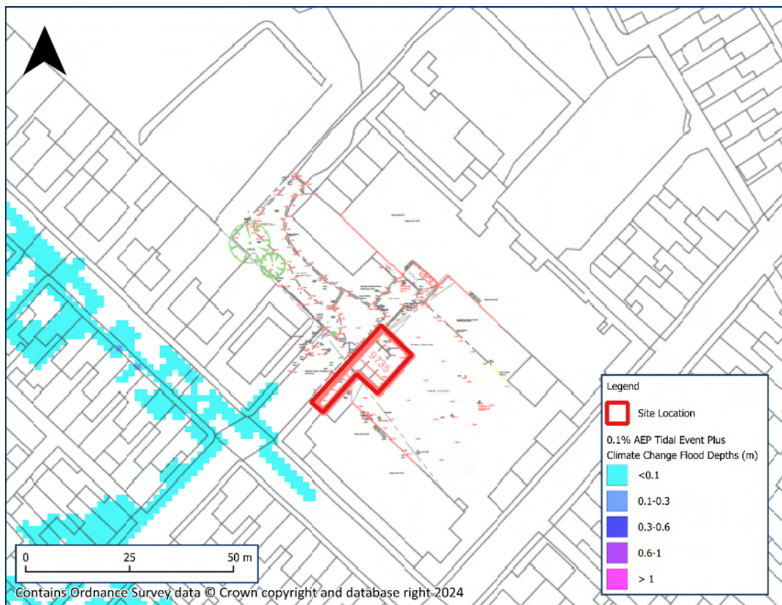
Figure 5-4 0.1% AEP Tidal Event Plus Climate Change Flood Depths
