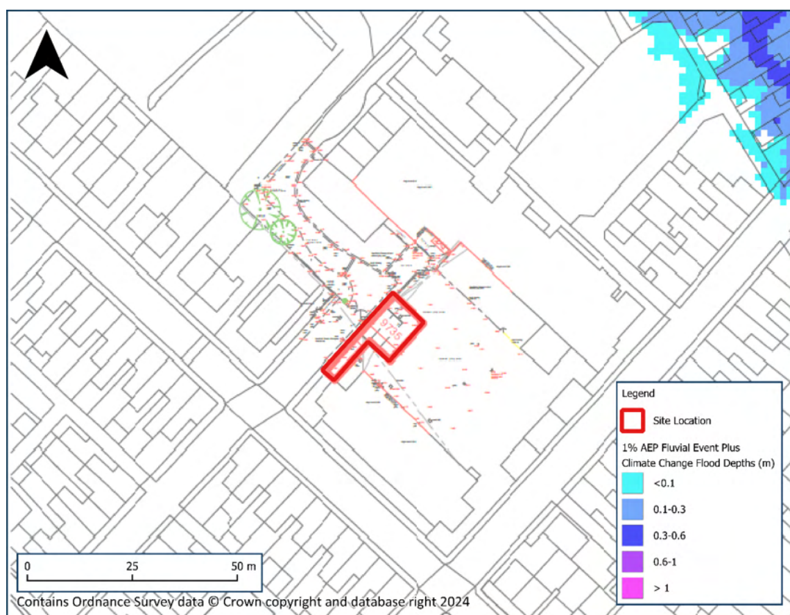
Figure 5-1 1% AEP Fluvial Event Plus Climate Change Flood Depths
