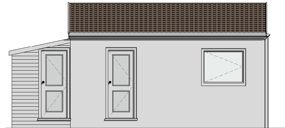
Left Elevation on Garage 1 : 50
