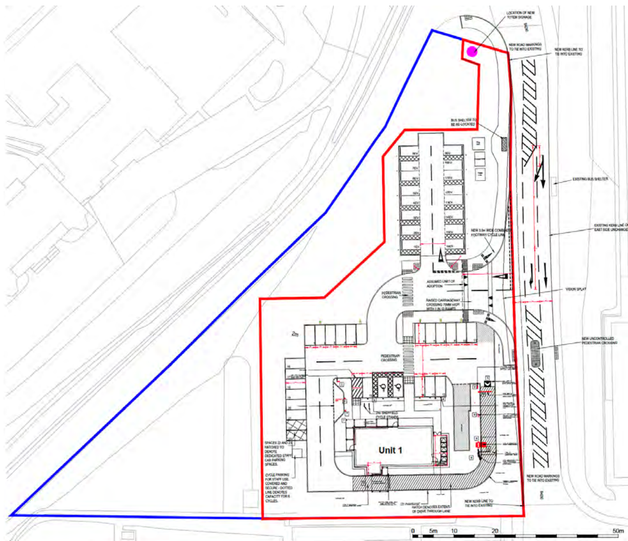
Figure 8 – Proposed Layout
