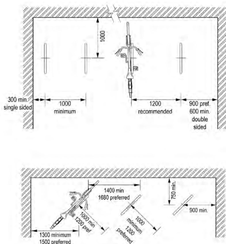
Figure 9 Active Travel Guidance Recommended Layouts and Dimensions of Cycle Stands
