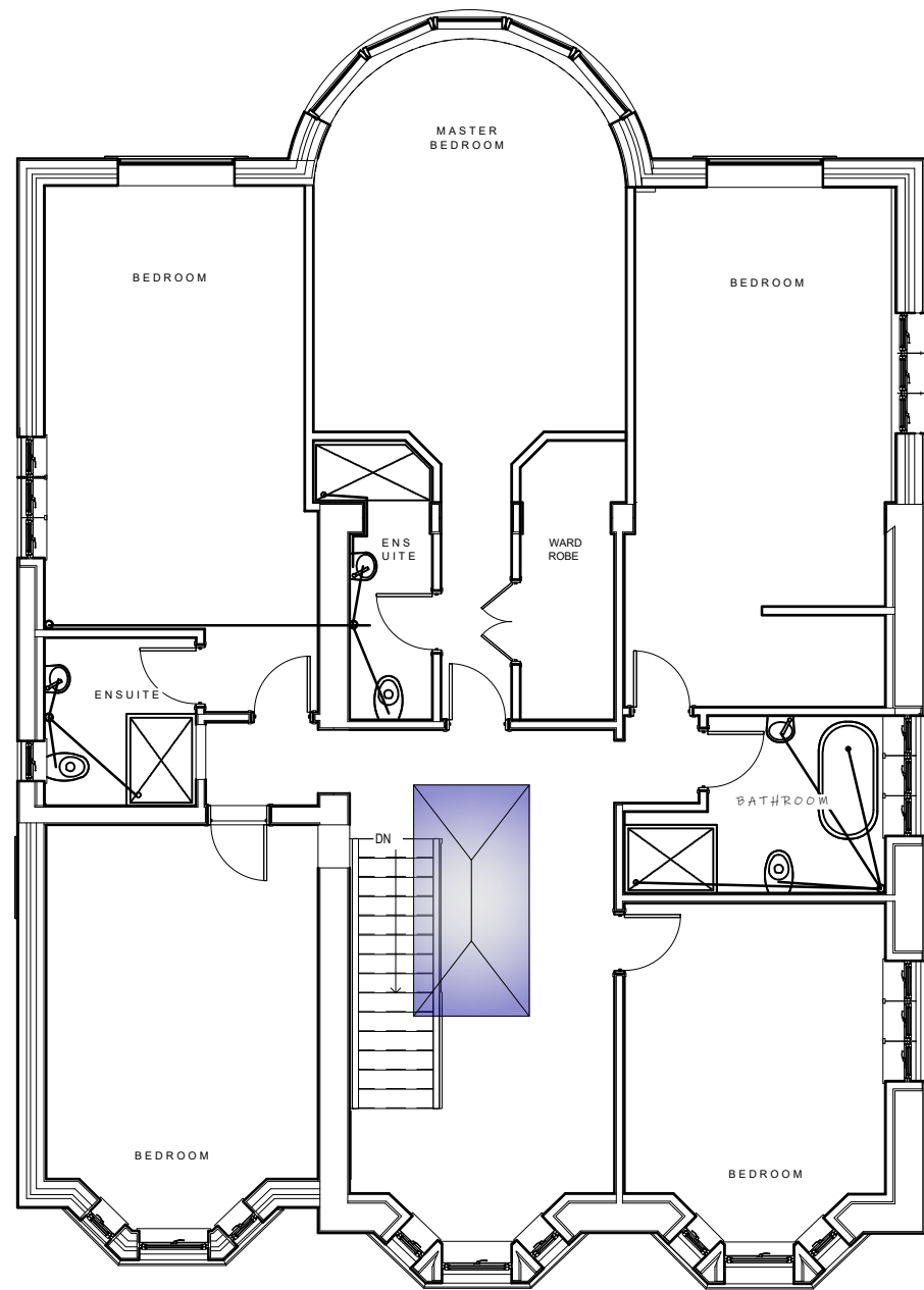
Proposed first floor layout Scale - 1:100
