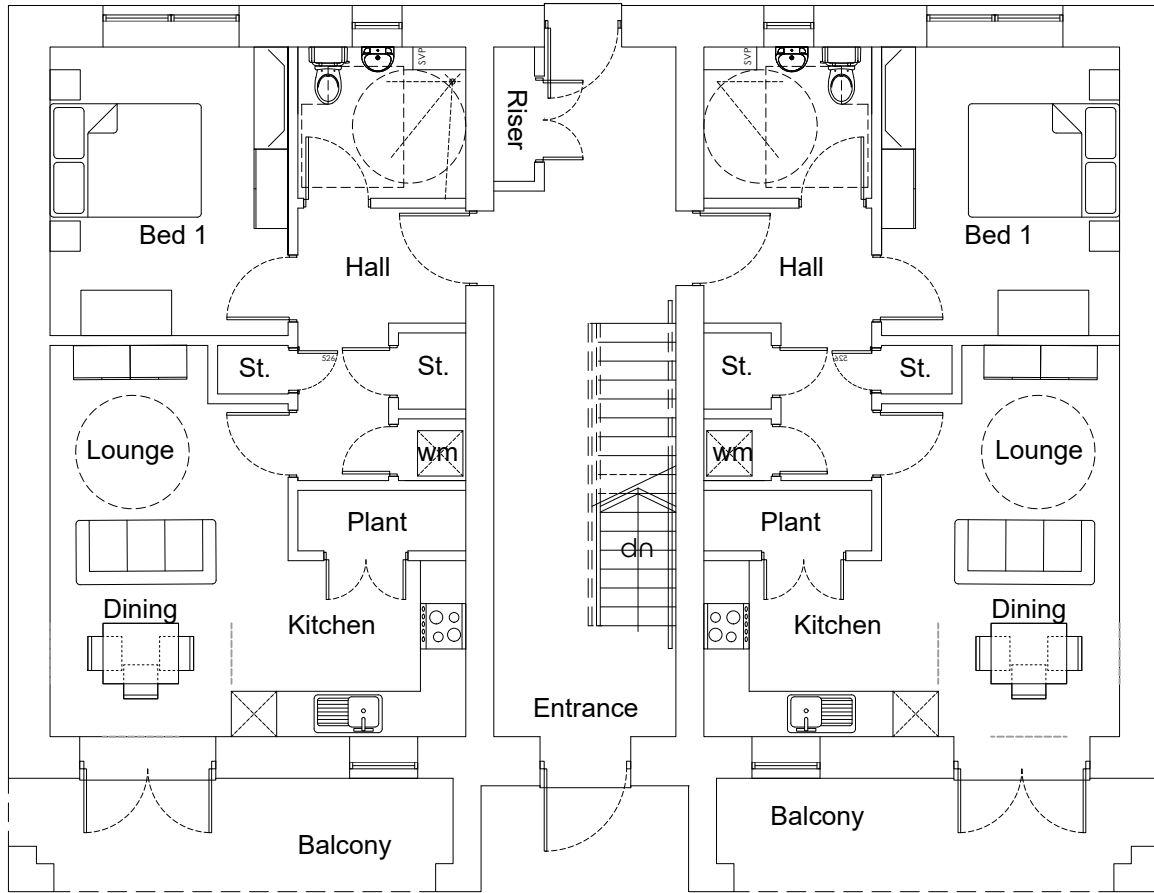
BUILDING TYPE D: GROUND FLOOR PLAN
