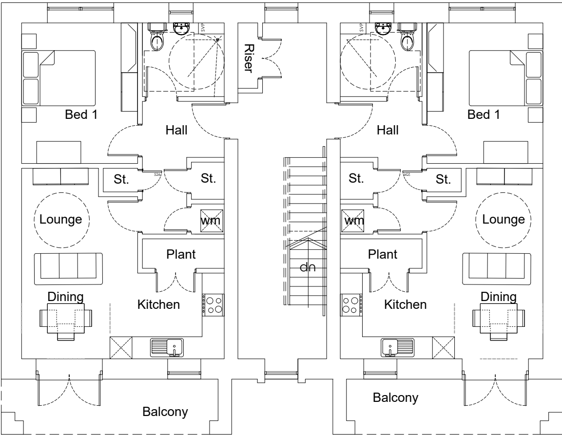
BUILDING TYPE D: FIRST FLOOR PLAN
