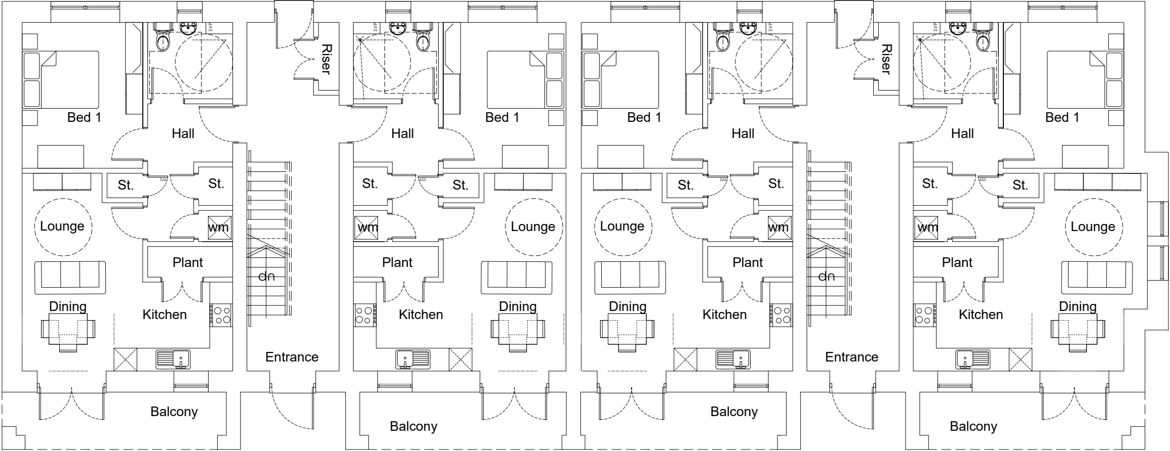
BUILDING TYPE C: GROUND FLOOR PLAN
