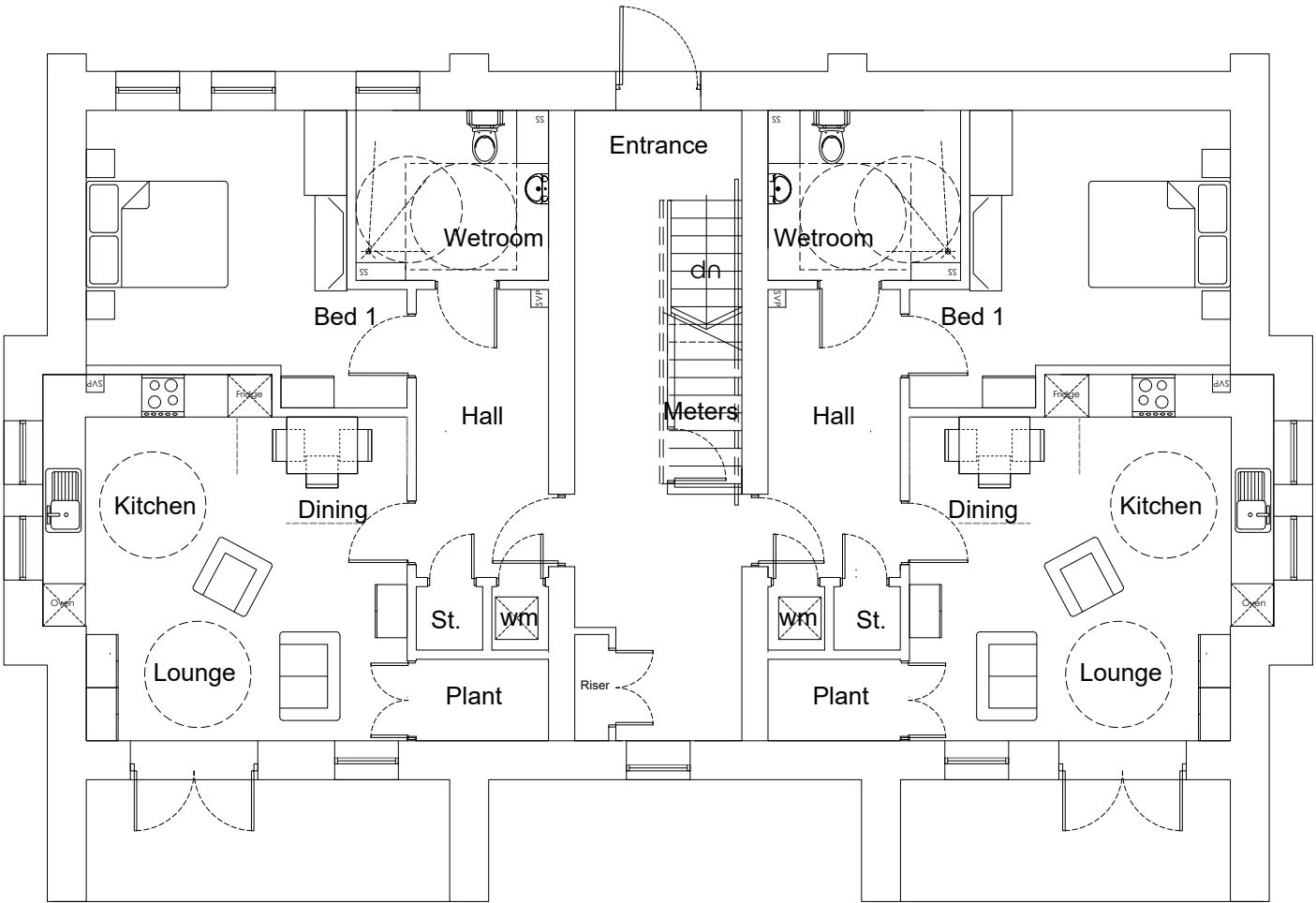
BUILDING TYPE A: GROUND FLOOR PLAN
