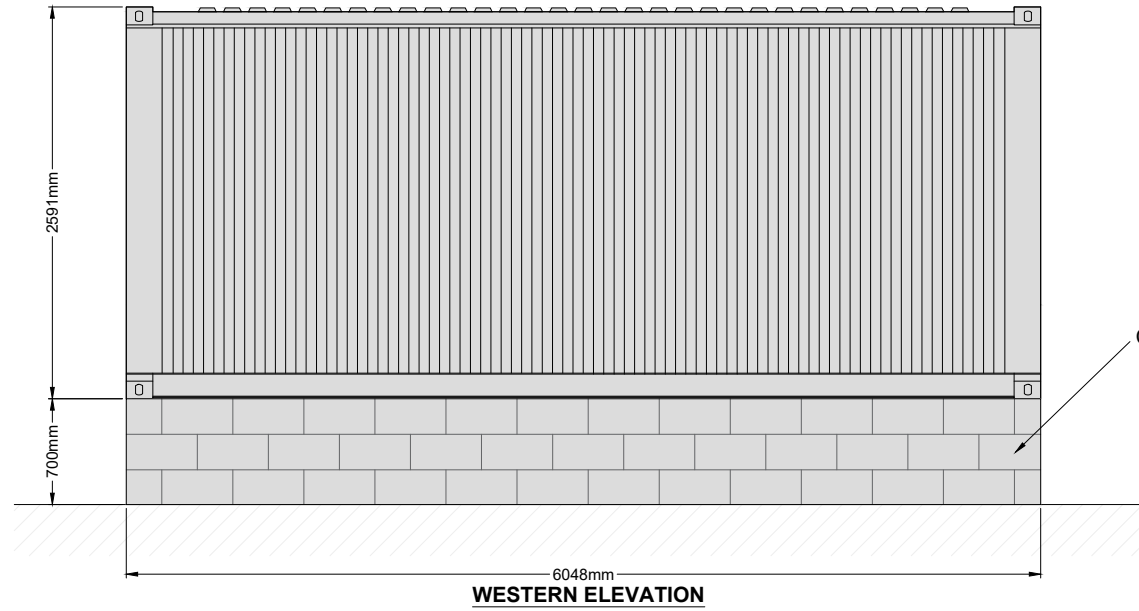
WESTERN ELEVATION
