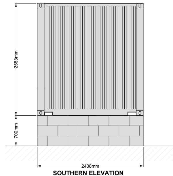
SOUTHERN ELEVATION
