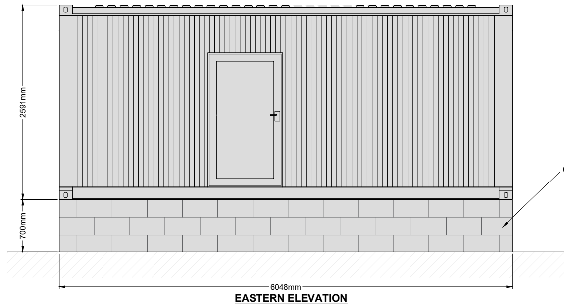
EASTERN ELEVATION
