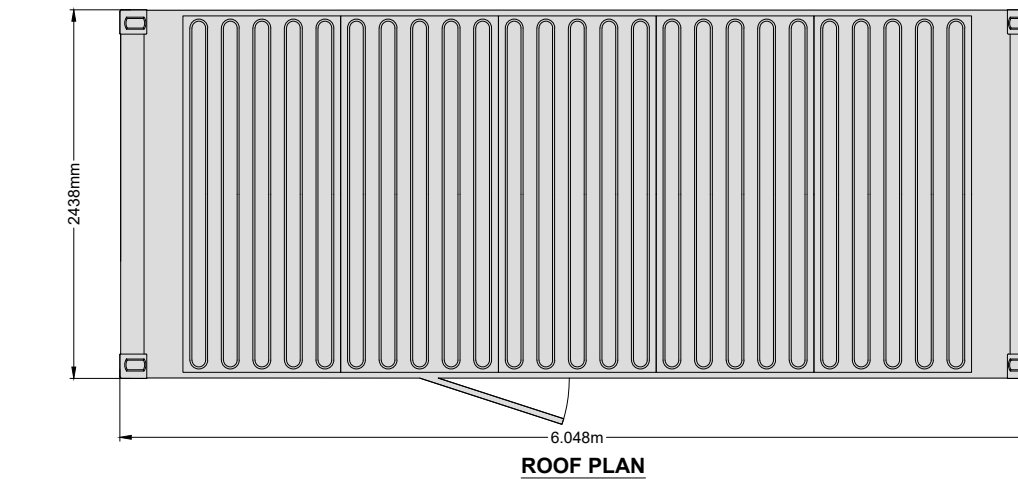
ROOF PLAN
