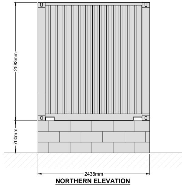
NORTHERN ELEVATION
