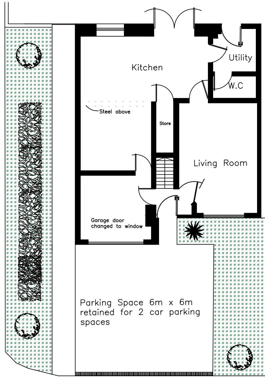
Proposed Floor/Block Plan 1:100
