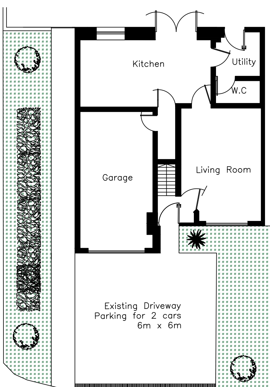
Existing Floor/Block Plan 1:100
