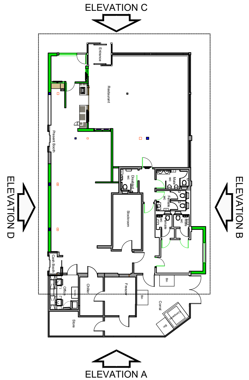
KEY PLAN 1:250
