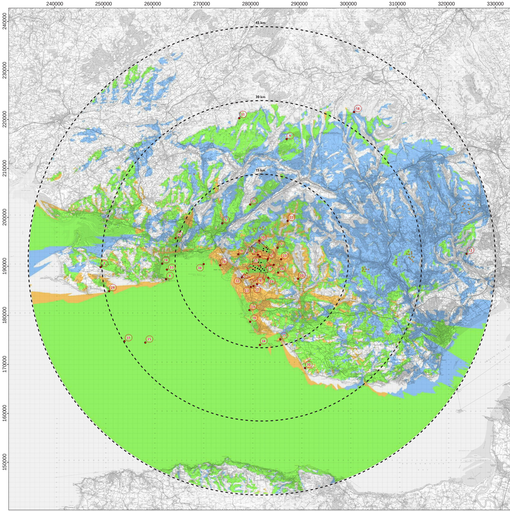
Title: Figure 8.12: 45 km Cumulative Wind Farm ZTV Scoping - Maximum Blade Tip Height
