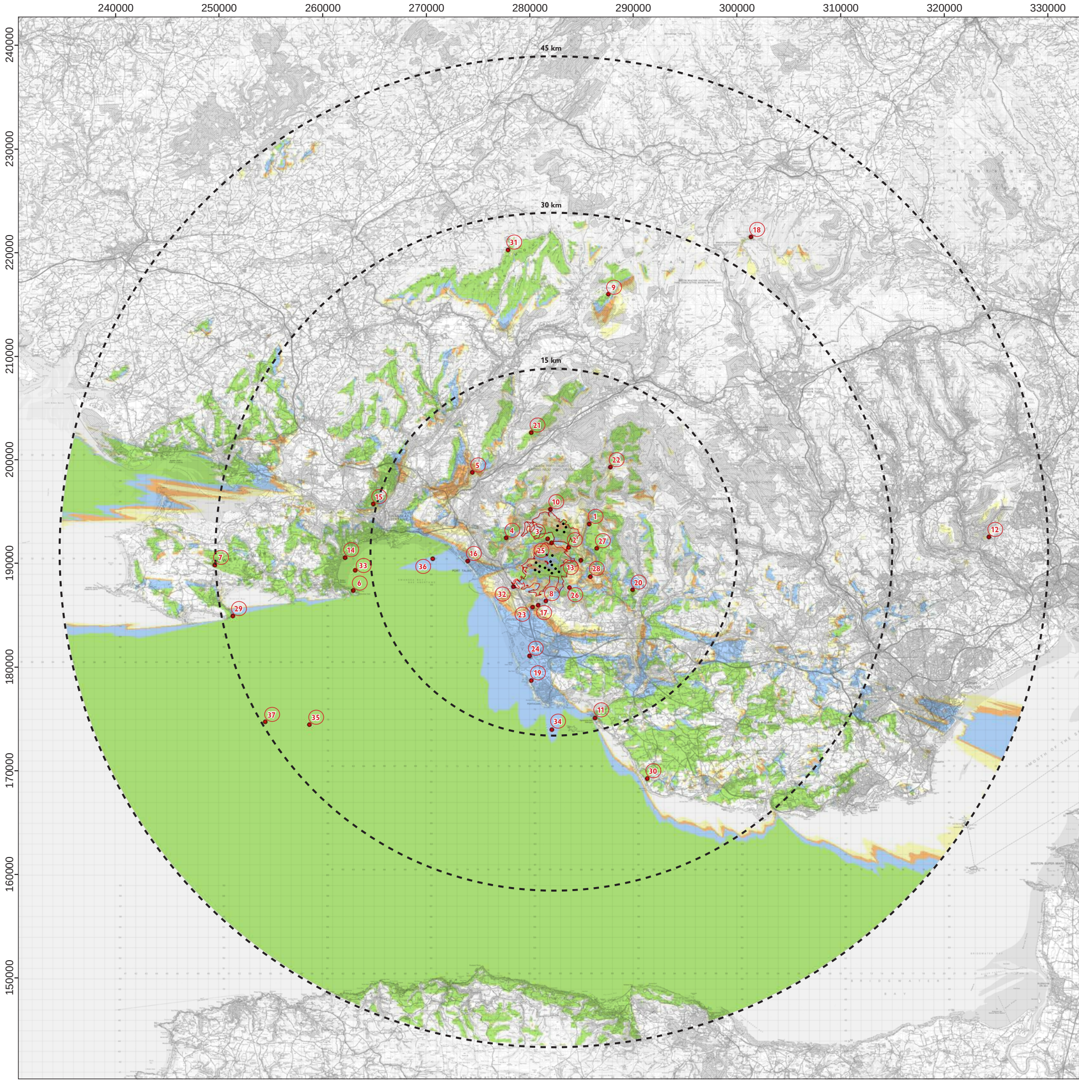
Title: Figure 8.3: 45 km Zone of Theoretical Visibility (ZTV) Maximum Hub Height
