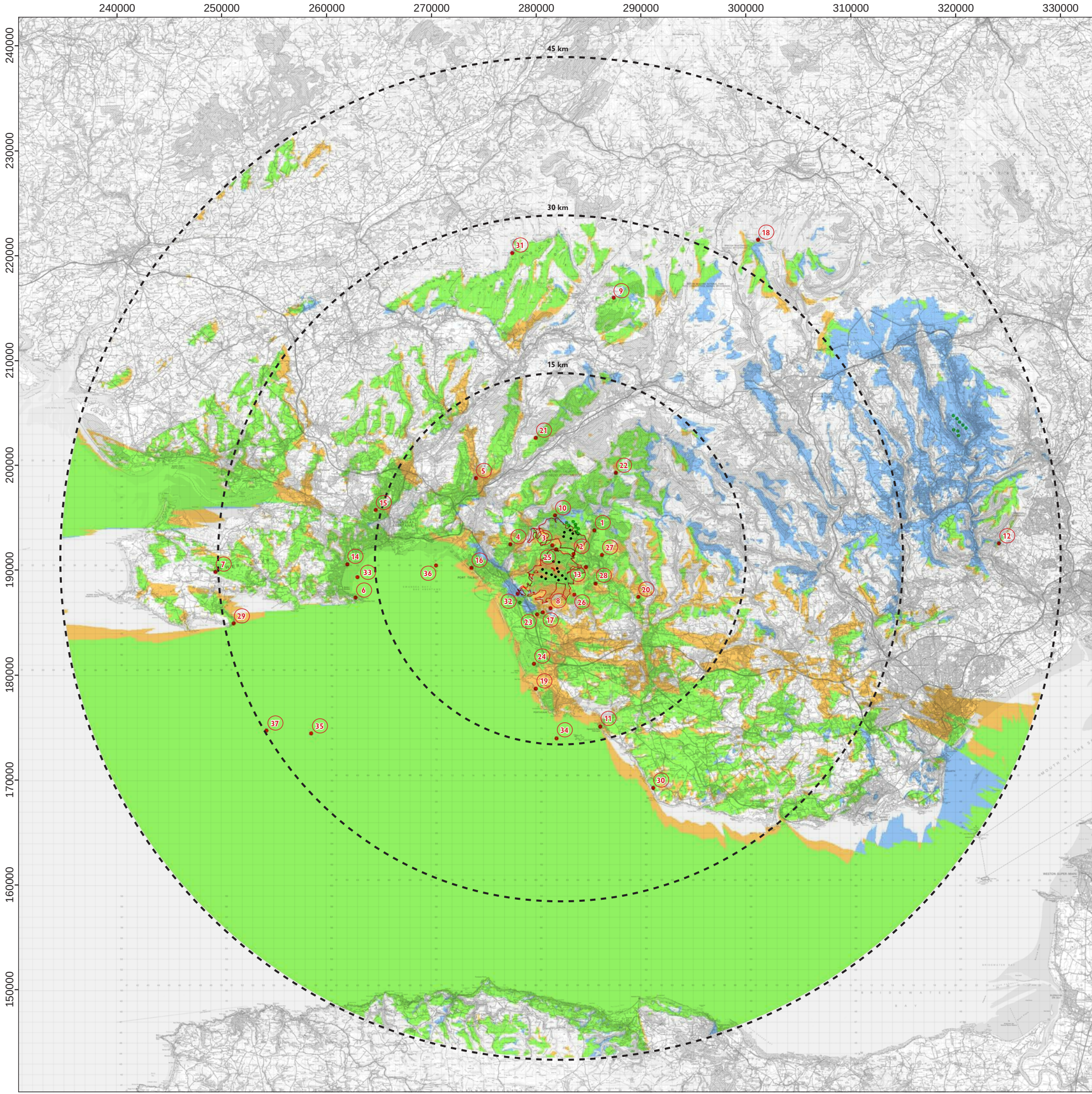
Title: Figure 8.10: 45 km Cumulative Wind Farm ZTV Submitted - Maximum Blade Tip Height
