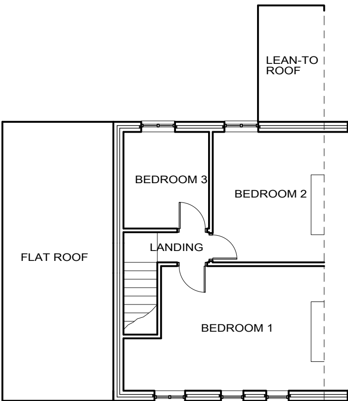
FIRST FLOOR PLAN EXISTING
