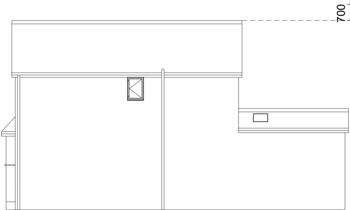
RIGHT SIDE ELEVATION EXISTING
