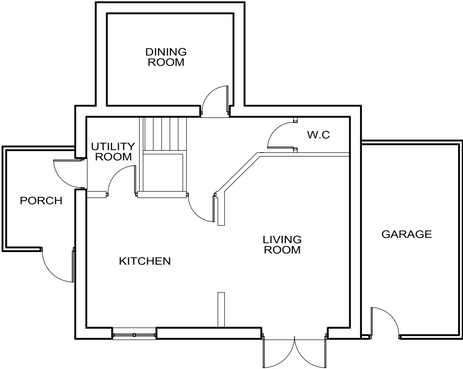
GROUND FLOOR PLAN EXISTING
