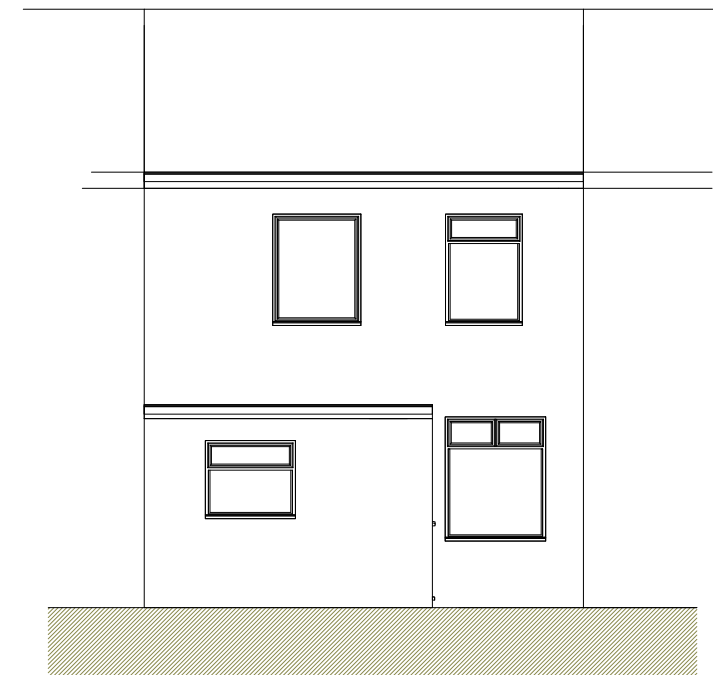
4 Rear Elevation 1 : 100
