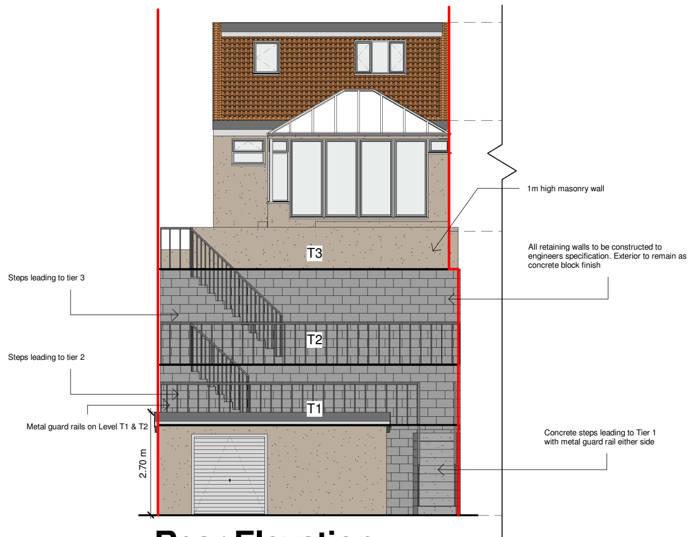
1 Rear Elevation 1 : 100
