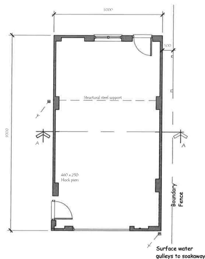
Proposed Garage Floorplan
