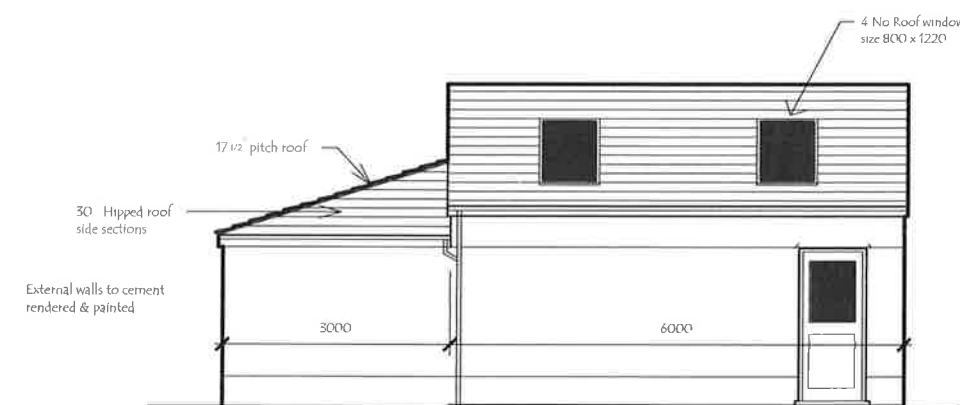
Side Elevation Facing East
