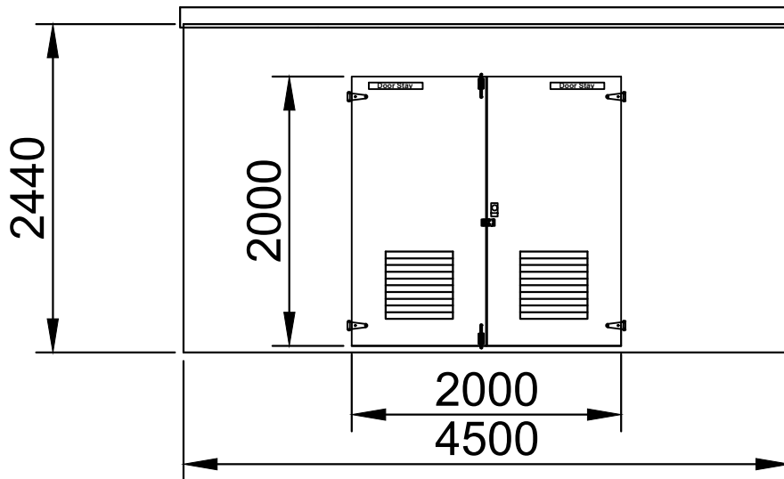
External Elevation WALL 1
