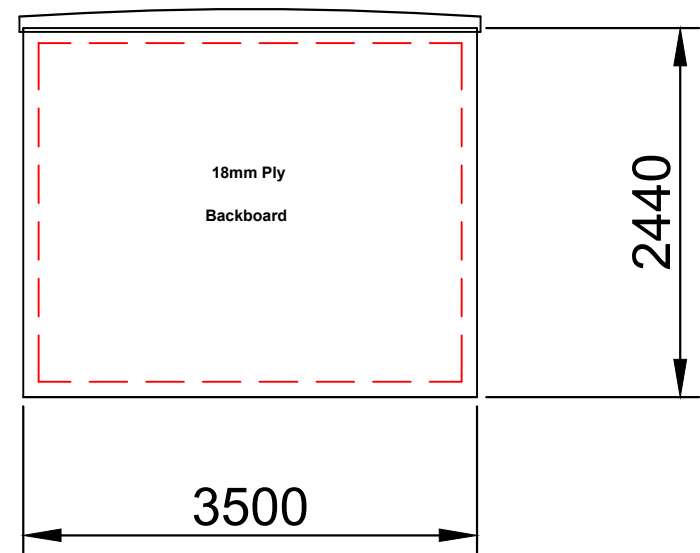
External Elevation WALL 4
