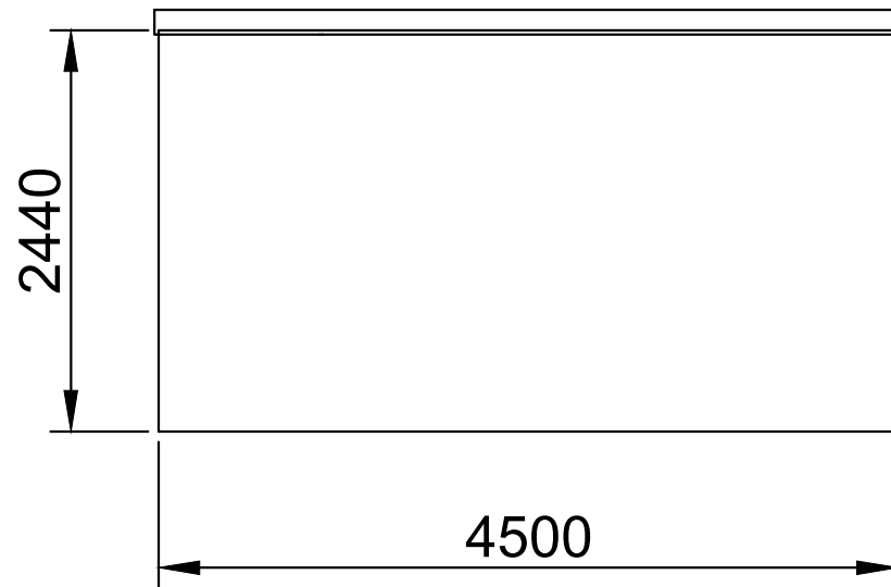
External Elevation WALL 3
