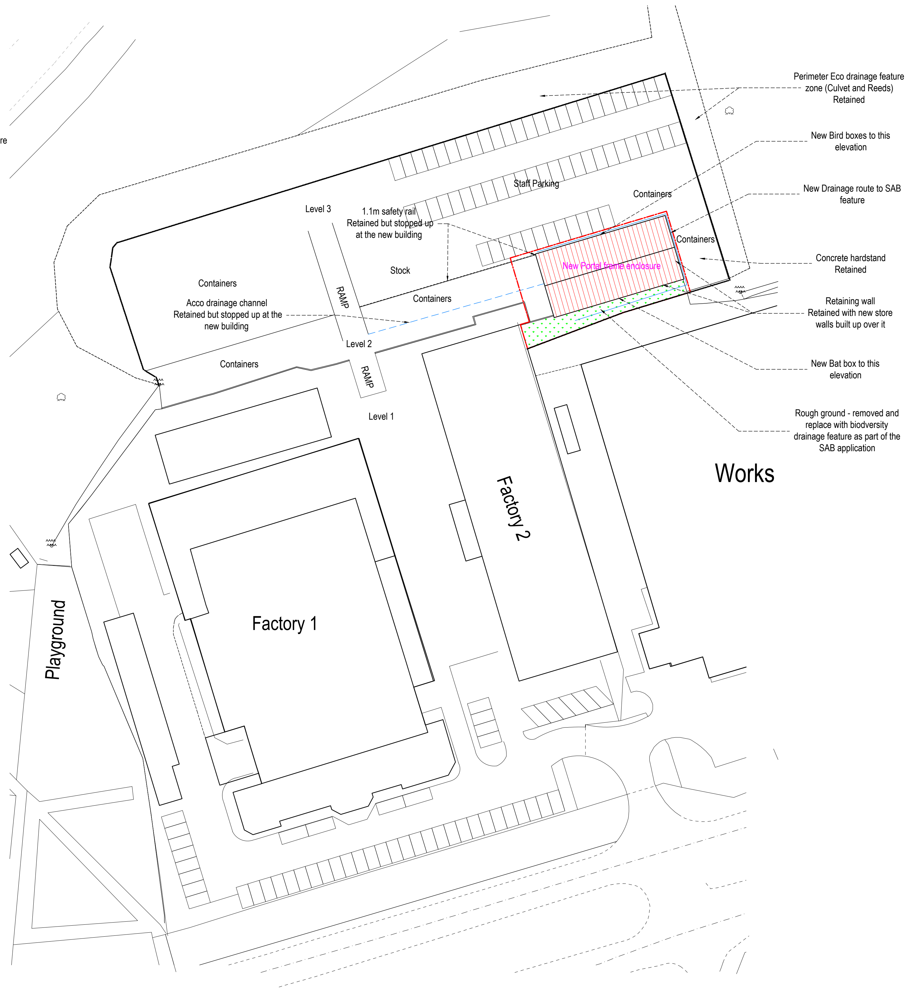
Proposed Site plan @ 1:500
