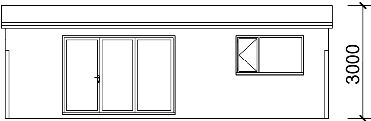
FRONT ELEVATION PROPOSED
