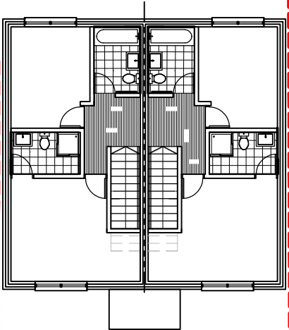
2 First Floor Plan Showing Obscured Glazing
