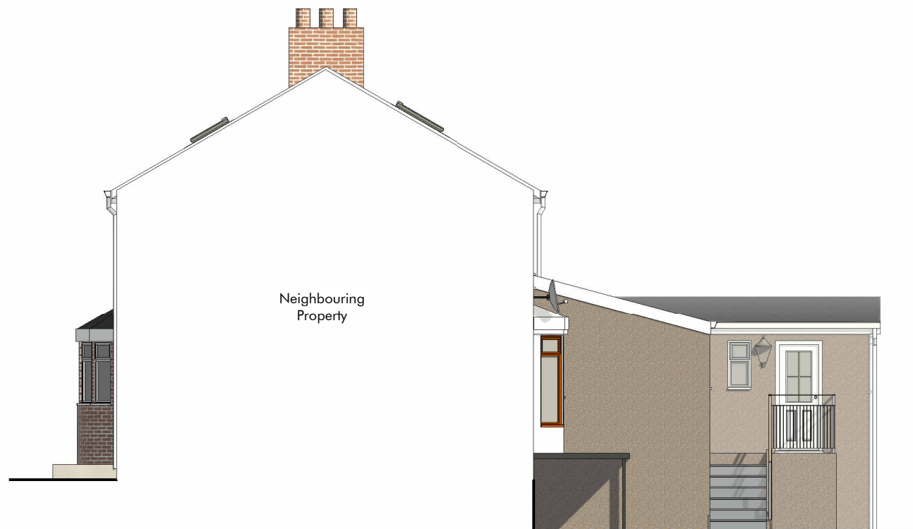
Side Elevation
