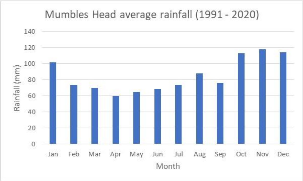
Figure 10.1.1: Average monthly rainfall data for climate period 1991-2020 for Mumbles Head Climate Station
