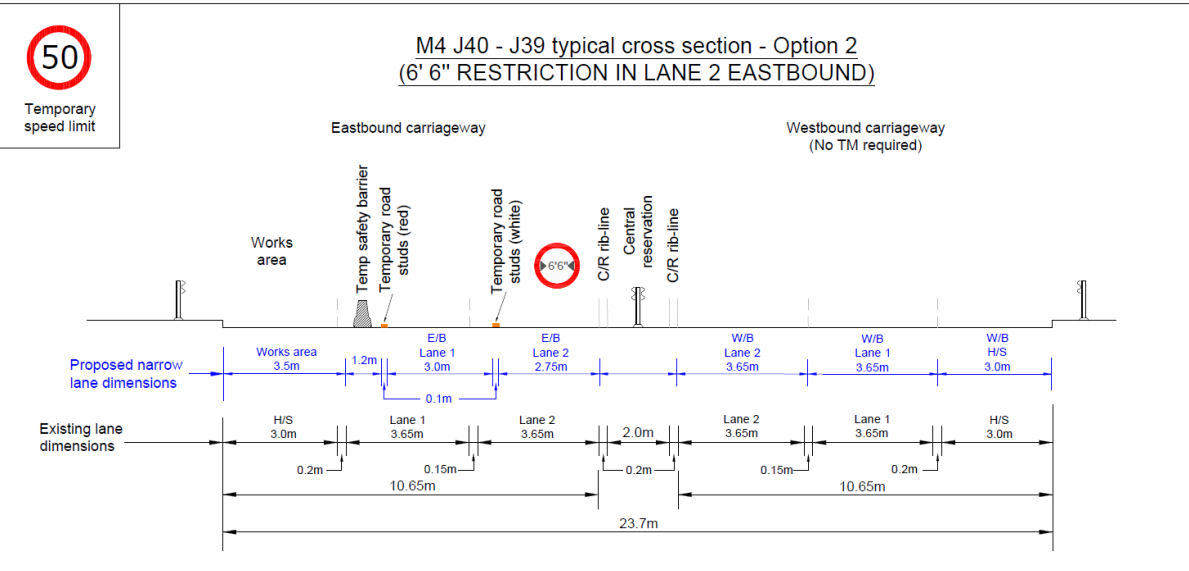
Figure 5.6.2 – Traffic management arrangement with width restriction to lane 2
