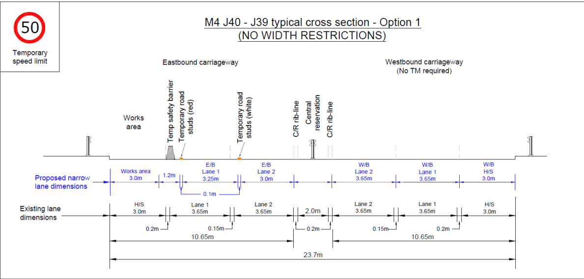
Figure 5.6.1: Narrow lanes traffic management cross section
